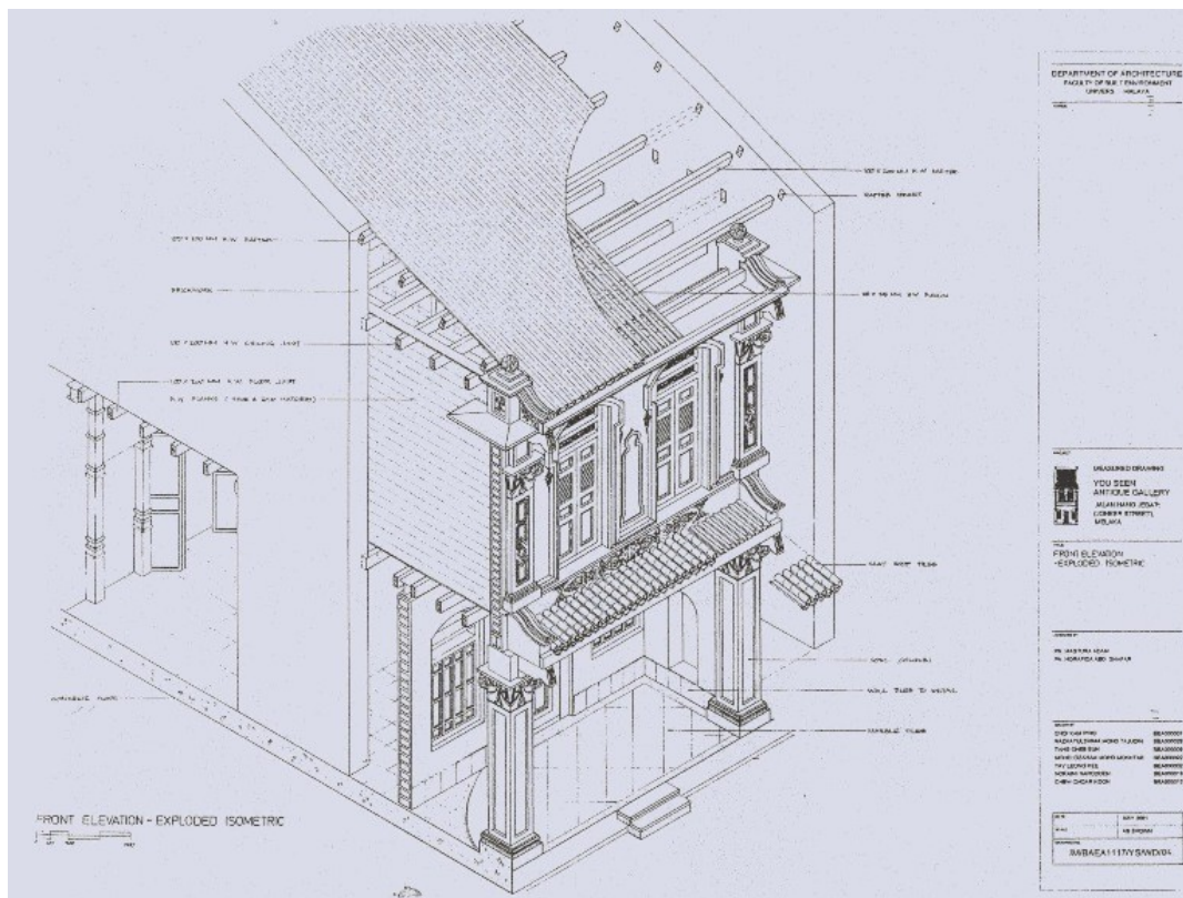
Mubin Sheppard Memorial Prize 2005 Category: Measured Drawings Winner: "You Seen Antique Gallery, Melaka (2001)"; Universiti Malaya
